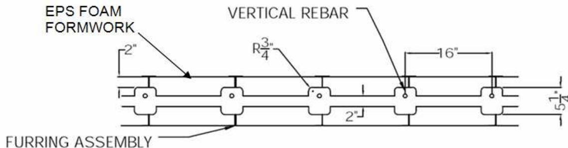
Figure 1. “HOBBS Wall” Composite Section
